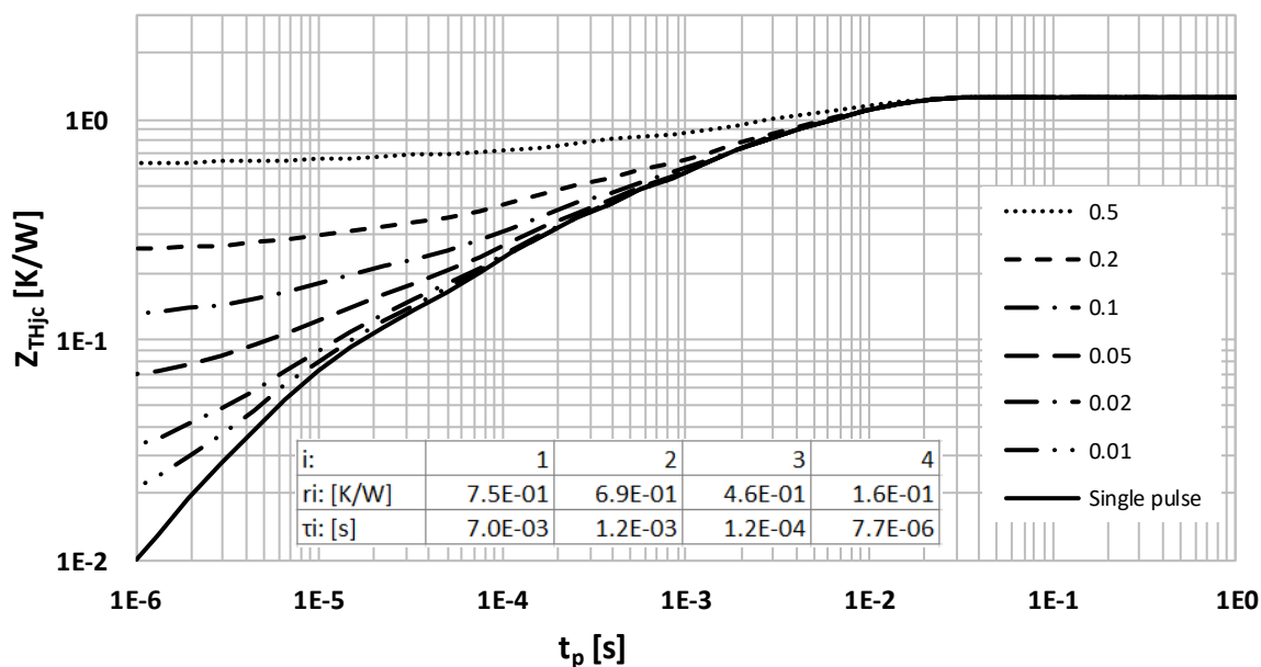
Figure 15 Max. transient thermal resistance (MOSFET)
