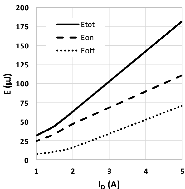
Figure 13 Typical switching energy losses as a function of drain-source current
