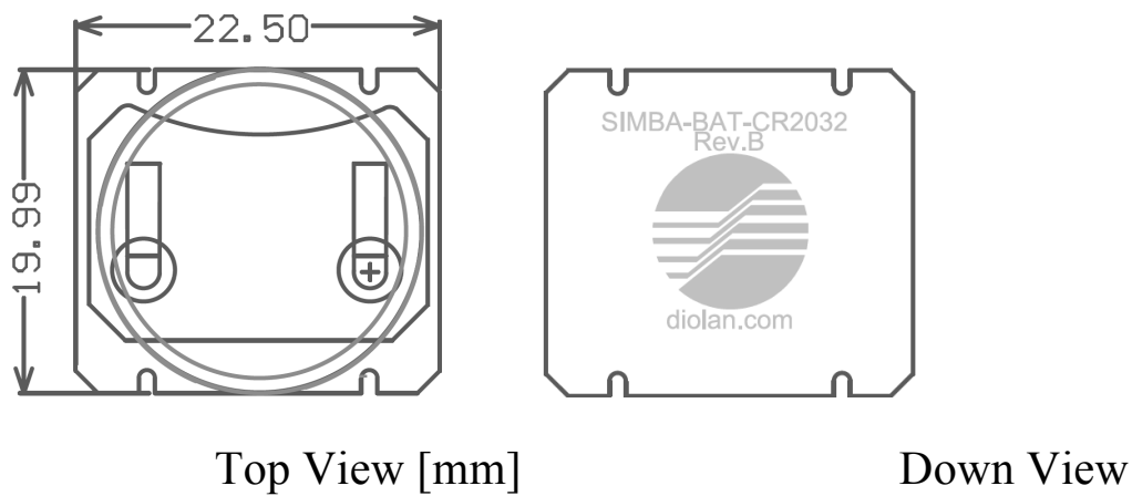
Figure 21 SensiBLE Battery Holder Top and Down View [mm]
