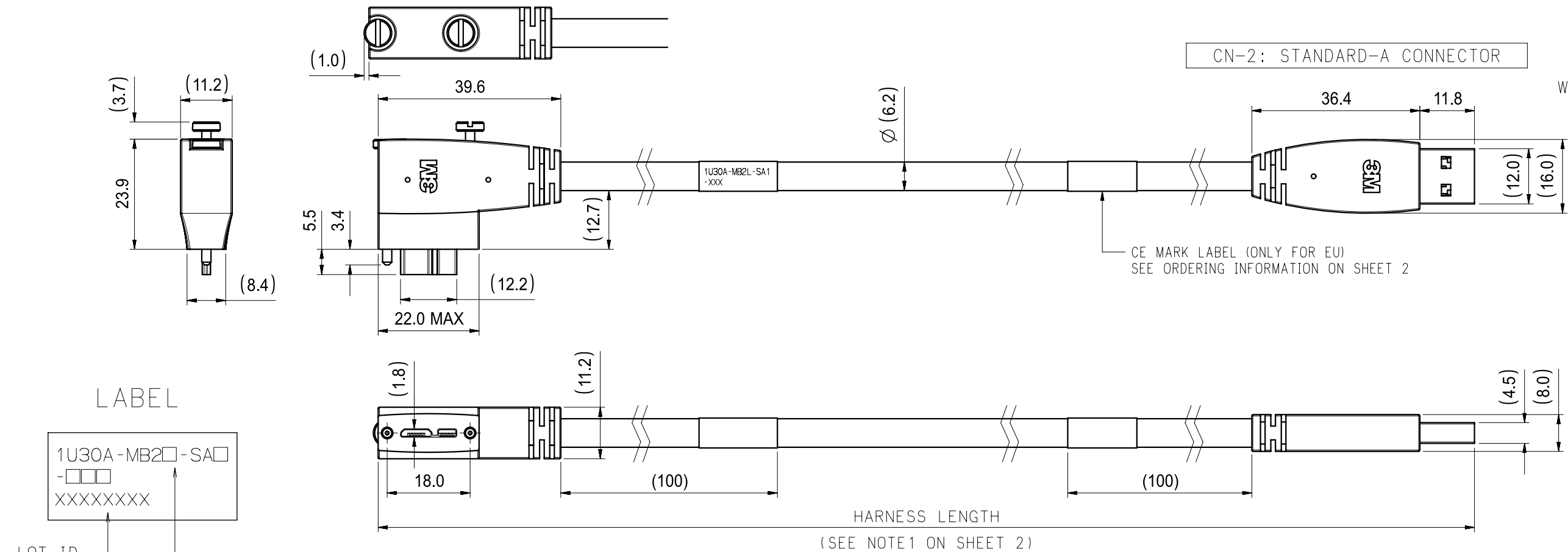
CN-1: MICRO-B CONNECTOR
