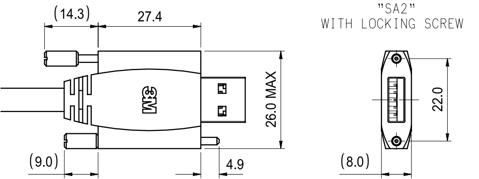
CN-2: STANDARD-A CONNECTOR
